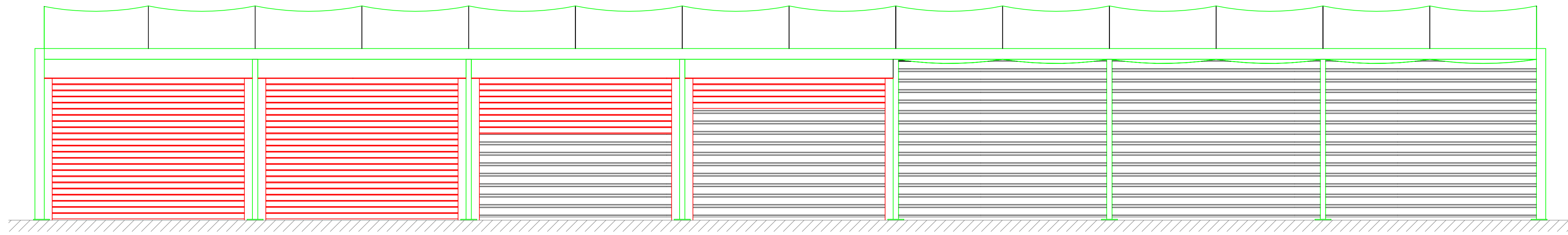
FRONT VIEW
