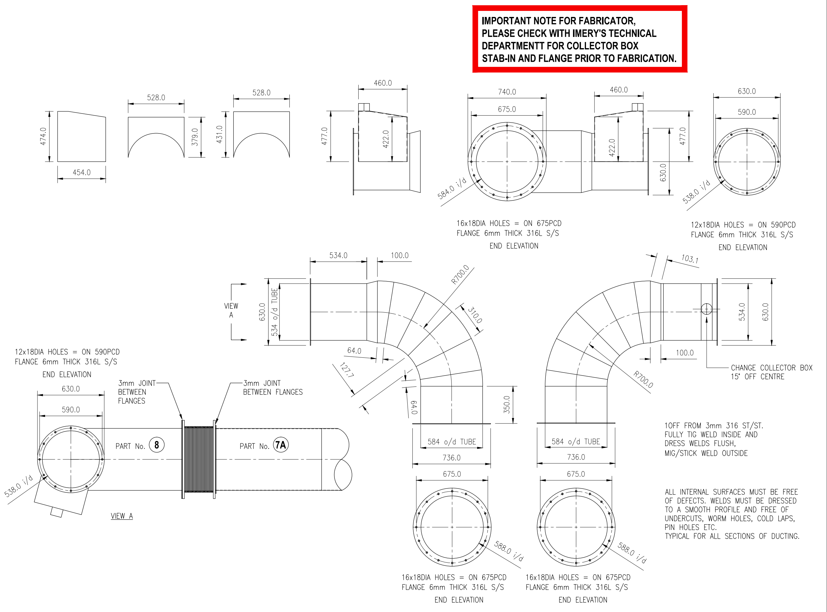
SIDE ELEVATION PART NUMBER 8
