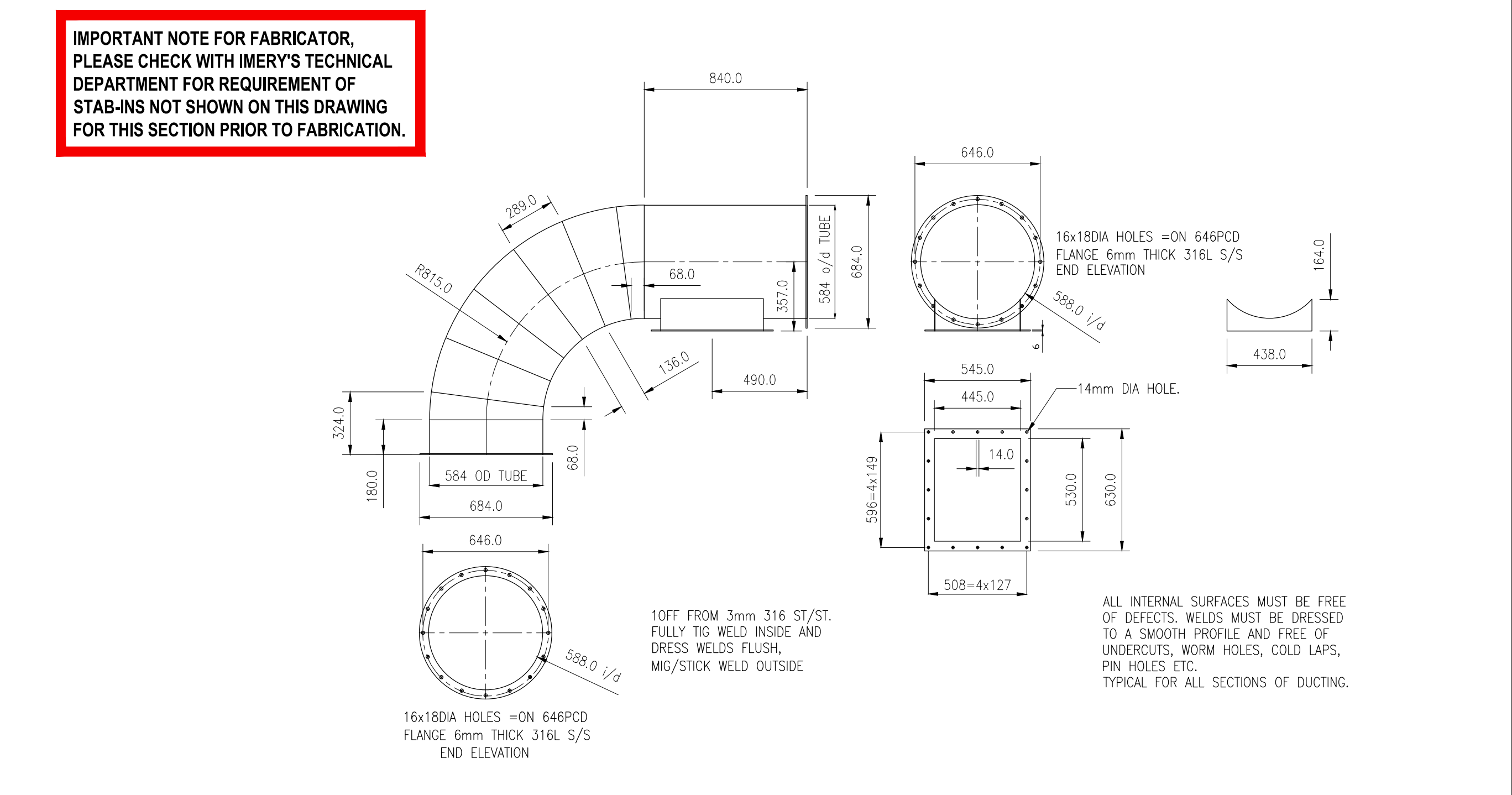
SIDE ELEVATION PART NUMBER 3
