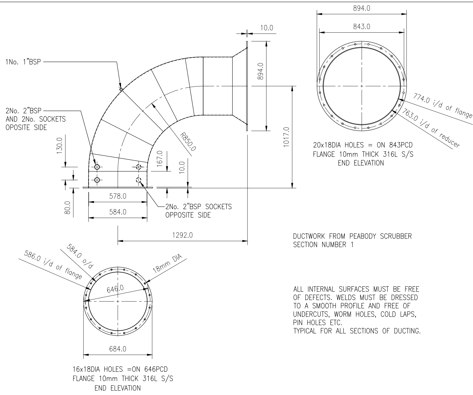
SIDE ELEVATION PART NUMBER 1
