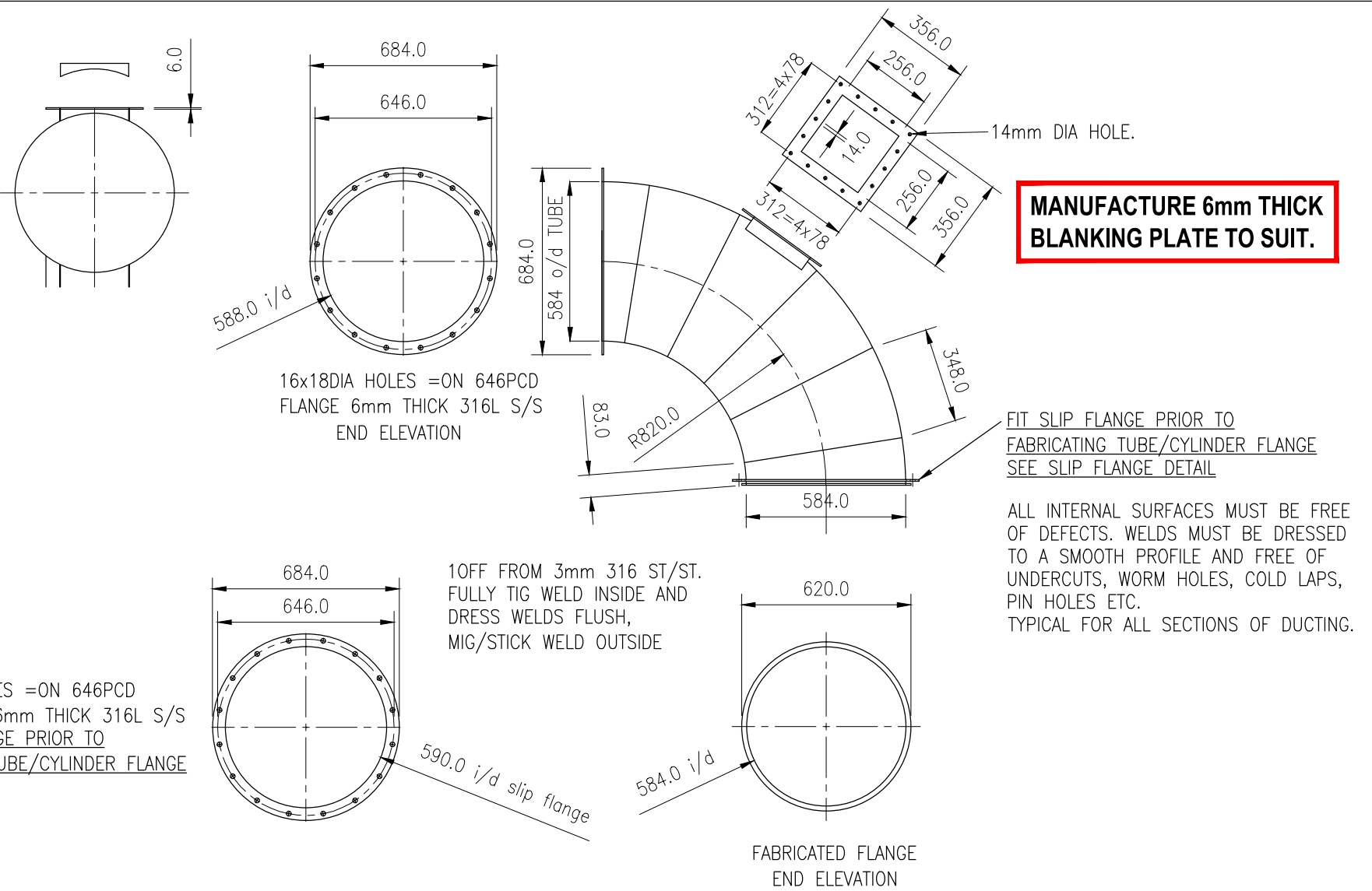
SIDE ELEVATION PART NUMBER 2
