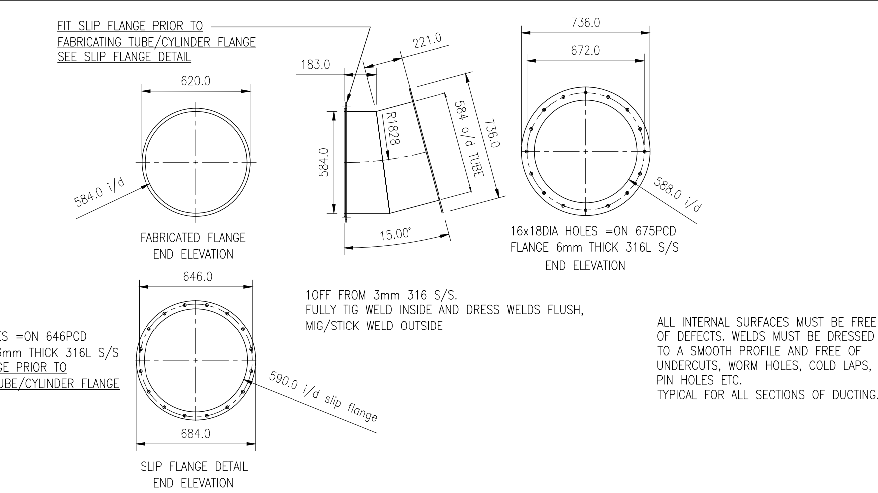
SIDE ELEVATION PART NUMBER 4
